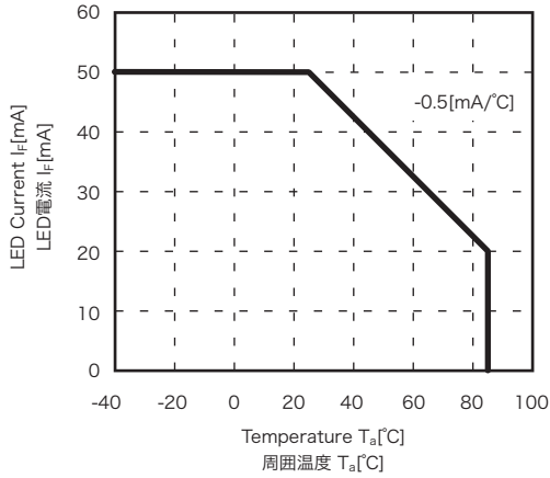
LED Current vs. Temperature LED電流-周囲温度特性
