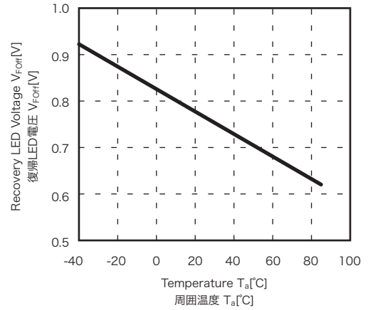
Recovery LED Voltage vs. Temperature 復帰LED電圧-周囲温度特性 ( V_L=60[V] , I_L=100[\mu A] )
