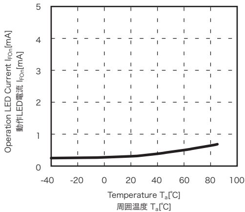
Operation LED Current vs. Temperature 動作LED電流-周囲温度特性 ( I_L=100[mA] )
