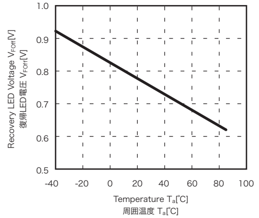
Recovery LED Voltage vs. Temperature 復帰LED電圧-周囲温度特性 ( V_L=80[V] , I_L=100[\mu A] )
