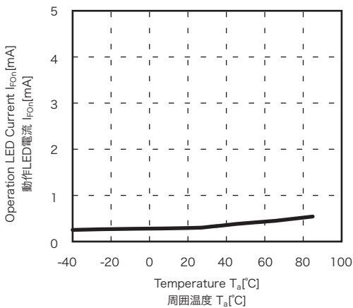
Operation LED Current vs. Temperature 動作LED電流-周囲温度特性 ( I_L=30[mA] )
