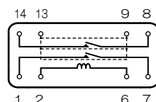
BOTTOM VIEW weight approximately 1.9gr.
