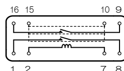
BOTTOM VIEW weight approximately 2.1gr.
